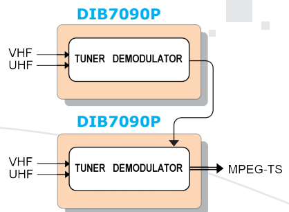
Diversity or dual reception architecture
